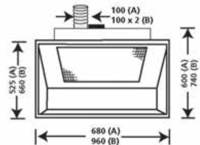
A Dimensions - BV200H-D B Dimensions - BV100H-D
