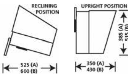
A Dimensions - BV300S B Dimensions - BV200S
