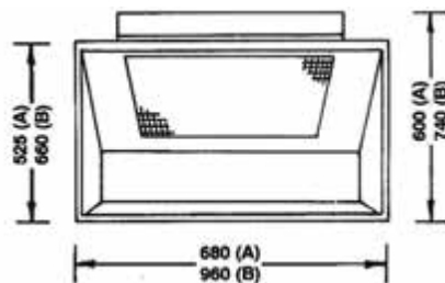
A Dimensions - BV200H B Dimensions - BV100H
